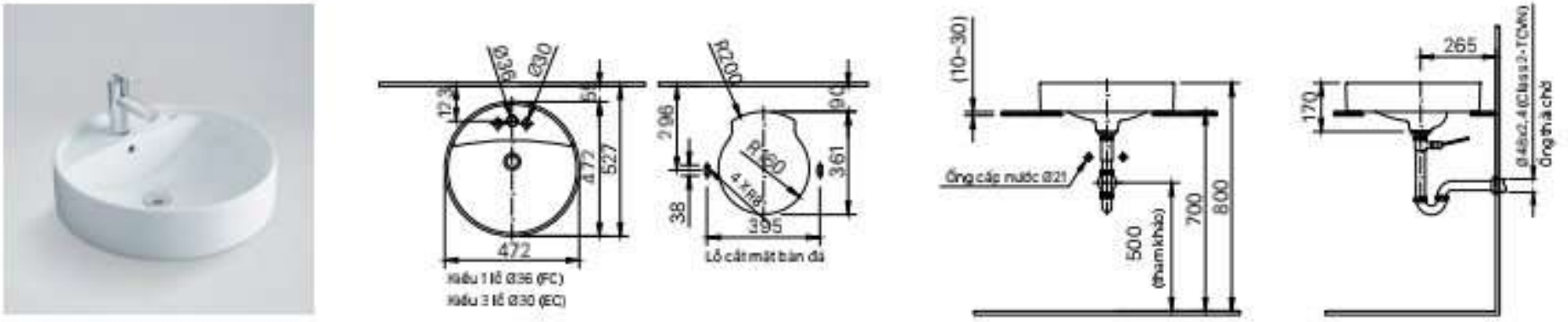
AL-294V (EC/FC) | L-294V (EC/FC)
