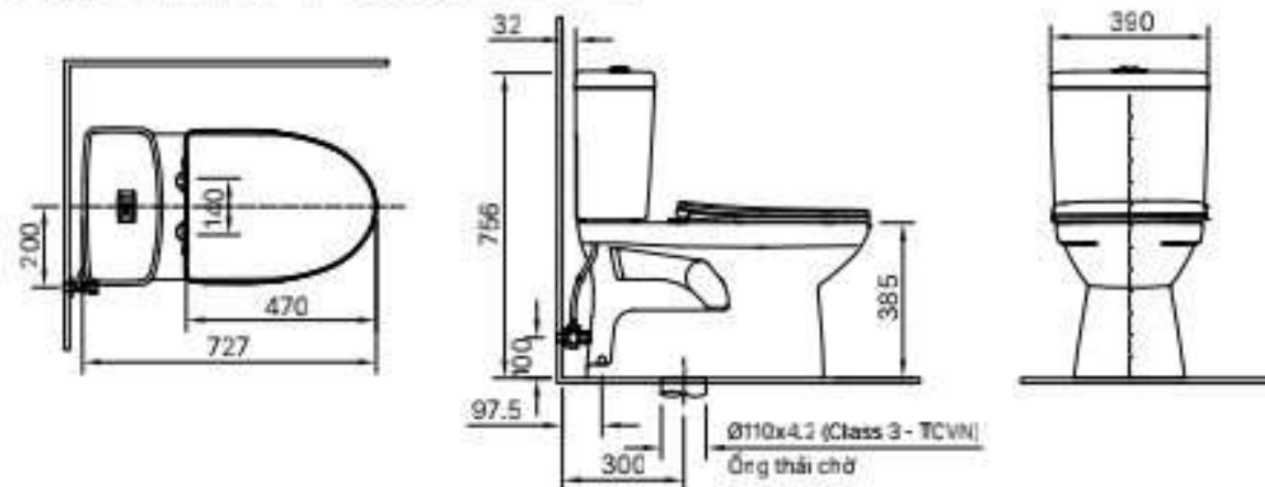
AC-504VAN-2 | C-504VAN-2 | AC-504VWN-2 | C-504VWN-2
