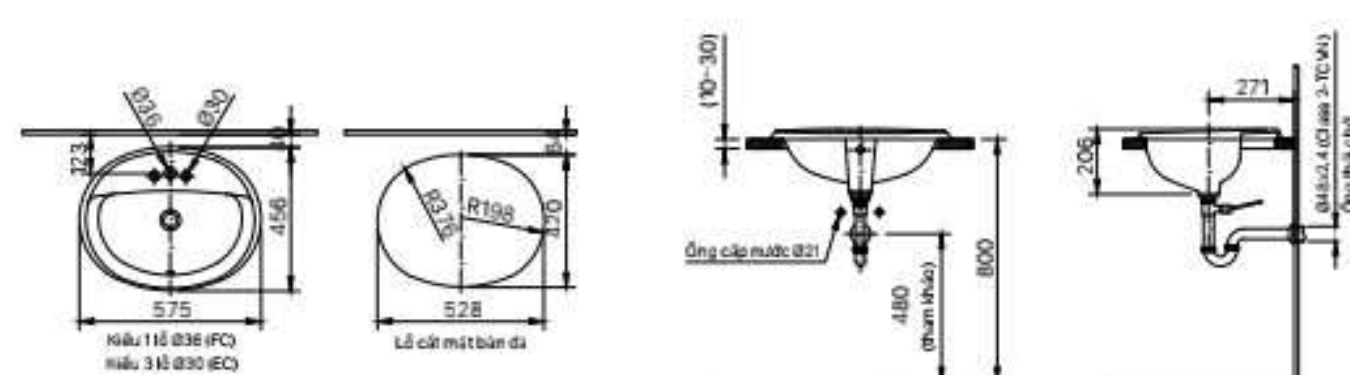
AL-2395V (EC/FC) | L-2395V (EC/FC)
